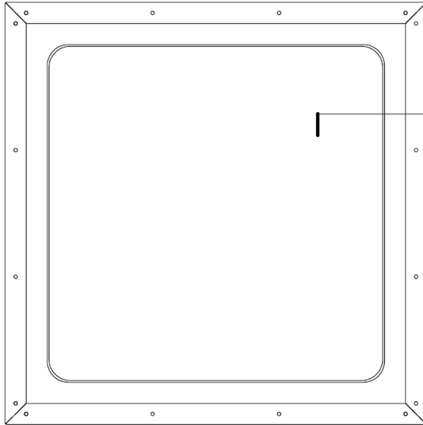
1 Typ. Access Panel Scale: NTS
